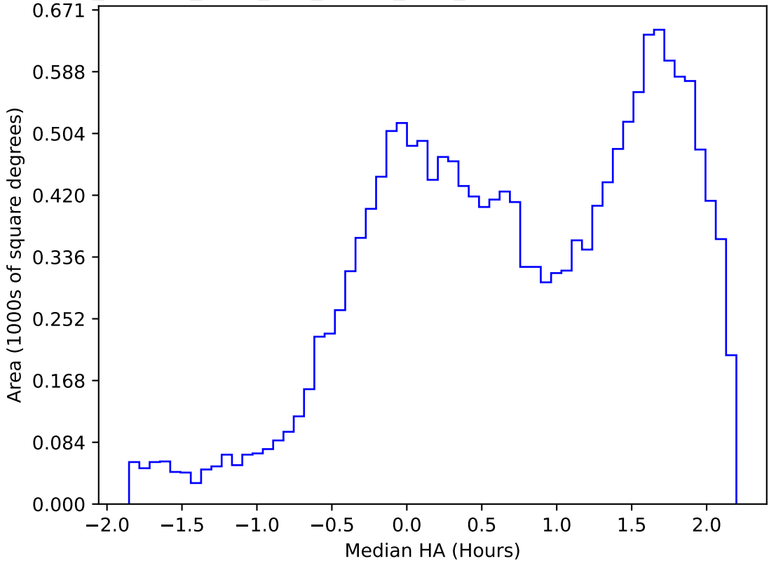
roll_uniform_early_half_mjdp0_v3.4_10yrs WFD u band: Median HA
