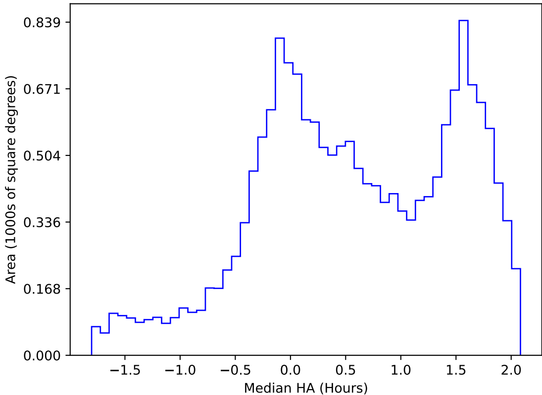
roll_uniform_early_half_mjdp0_v3.4_10yrs WFD g band: Median HA
