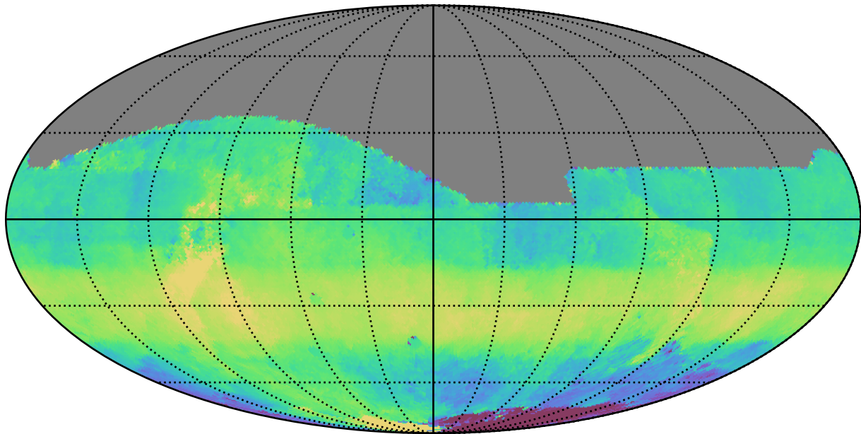
roll_uniform_early_half_mjdp0_v3.4_10yrs All sky z band: Median HA
