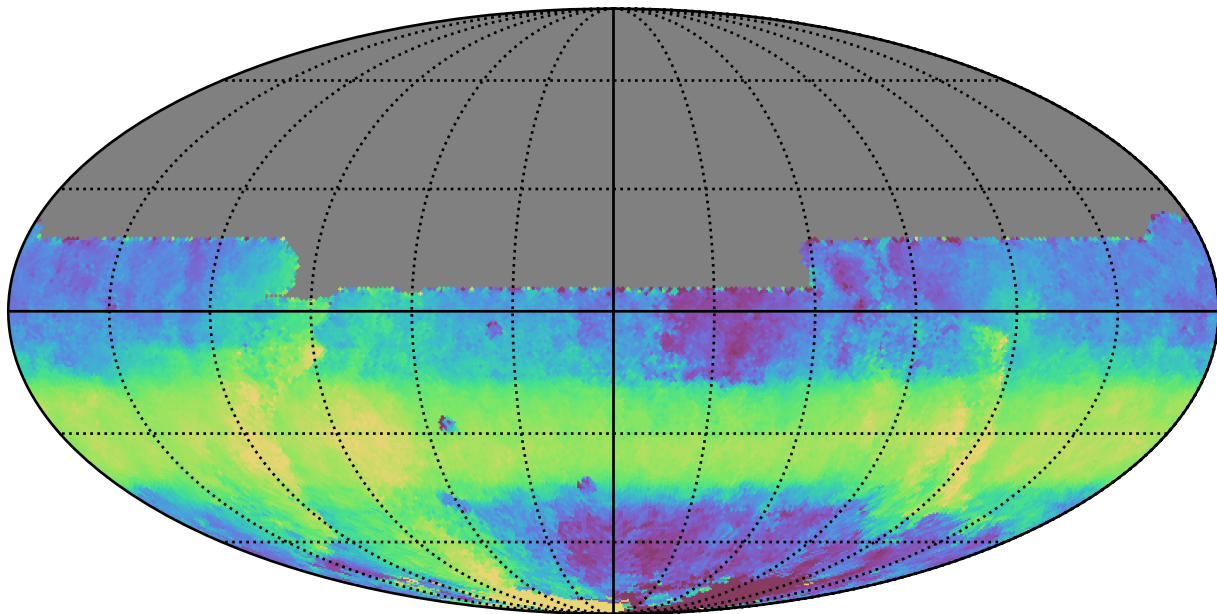
roll_uniform_early_half_mjdp0_v3.4_10yrs All sky y band: Median HA
