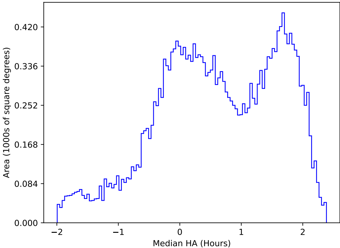
roll_uniform_early_half_mjdp0_v3.4_10yrs All sky u band: Median HA
