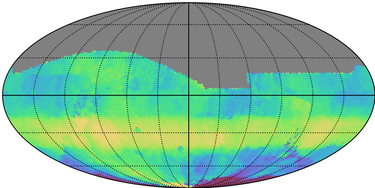
roll_uniform_early_half_mjdp0_v3.4_10yrs All sky r band: Median HA
