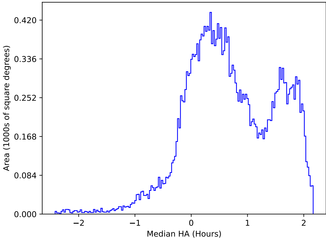
roll_uniform_early_half_mjdp0_v3.4_10yrs All sky r band: Median HA
