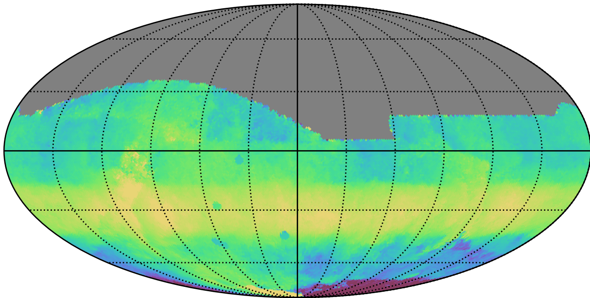
roll_uniform_early_half_mjdp0_v3.4_10yrs All sky i band: Median HA
