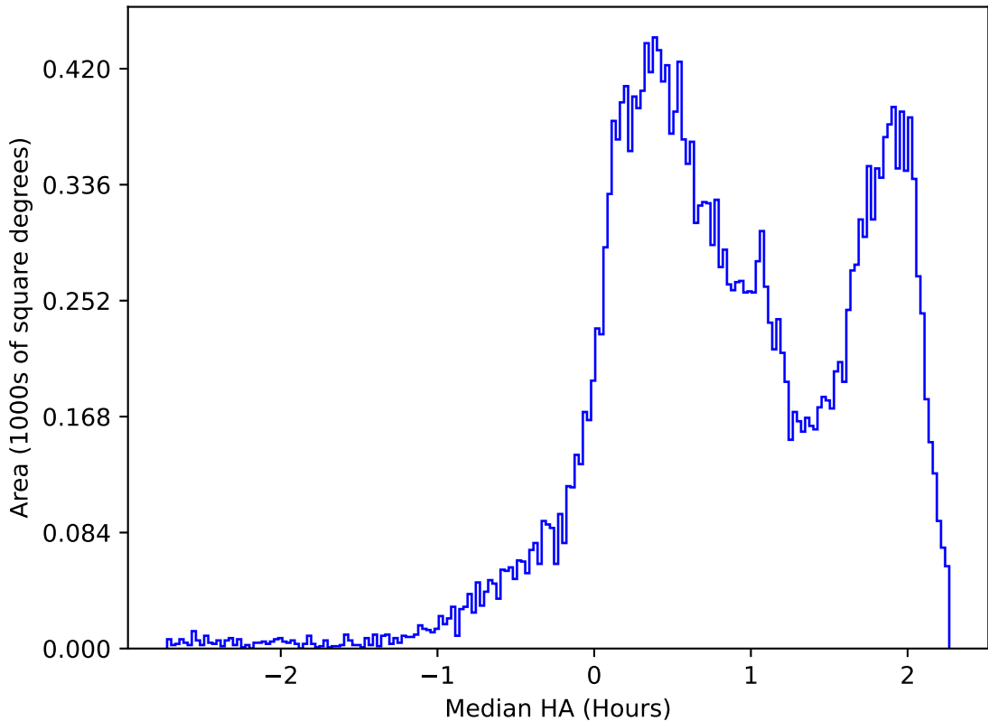
roll_uniform_early_half_mjdp0_v3.4_10yrs All sky i band: Median HA
