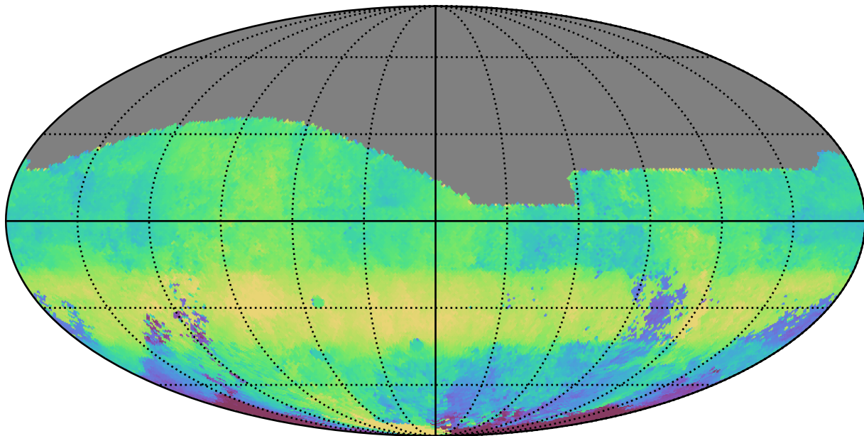
roll_uniform_early_half_mjdp0_v3.4_10yrs All sky g band: Median HA
