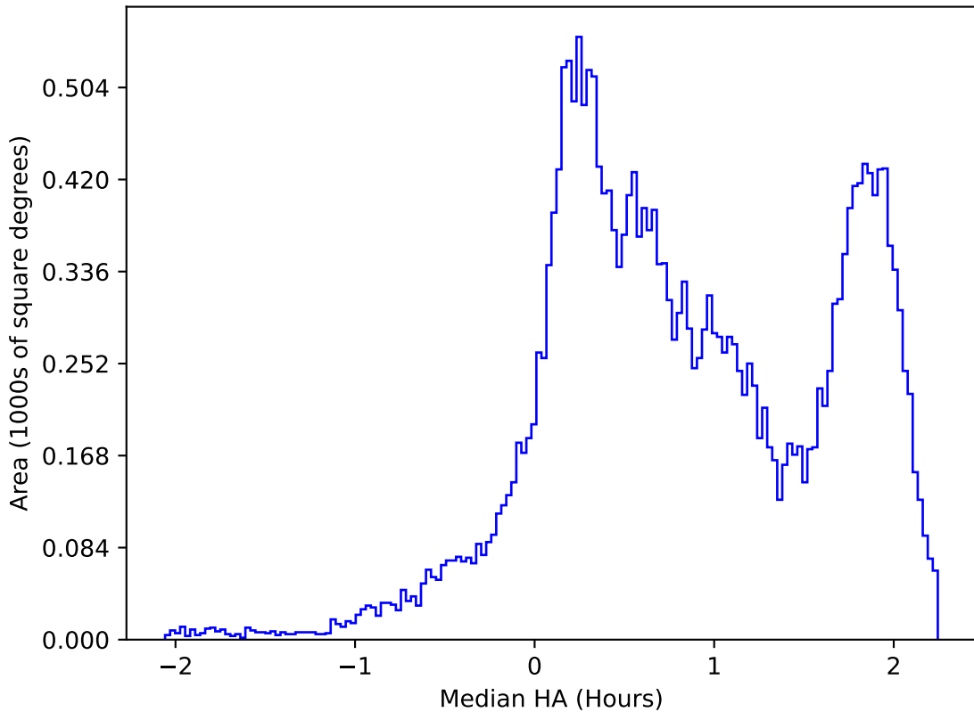
roll_uniform_early_half_mjdp0_v3.4_10yrs All sky all bands: Median HA
