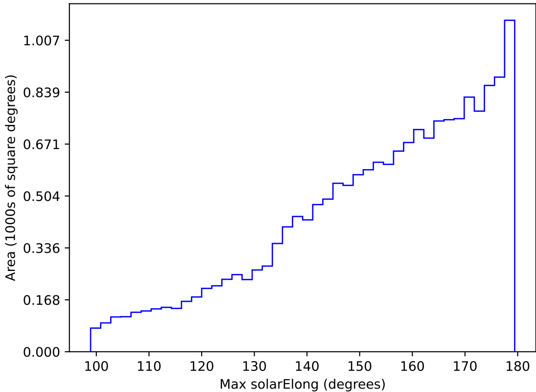
roll_uniform_early_half_mjdp0_v3.4_10yrs WFD r band: Max solarElong
