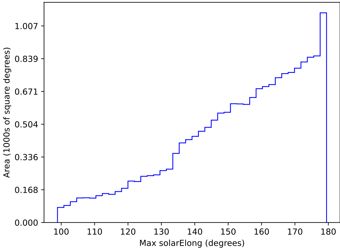
roll_uniform_early_half_mjdp0_v3.4_10yrs WFD i band: Max solarElong
