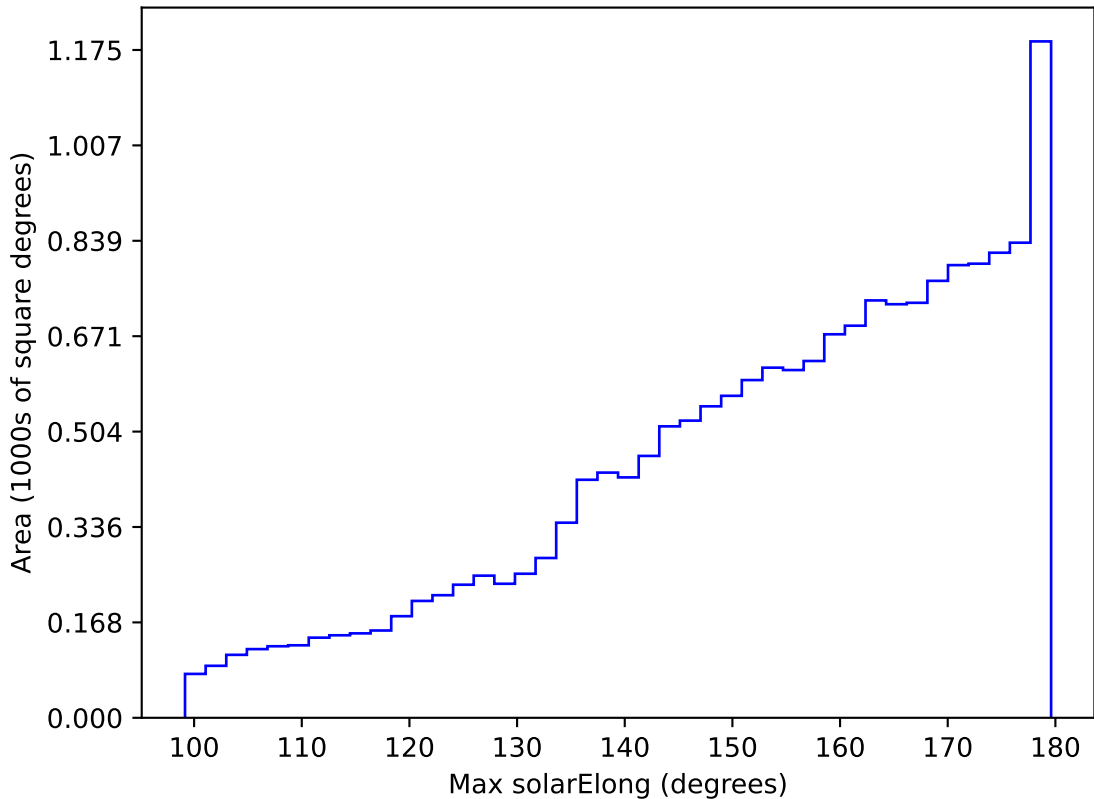
roll_uniform_early_half_mjdp0_v3.4_10yrs WFD all bands: Max solarElong
