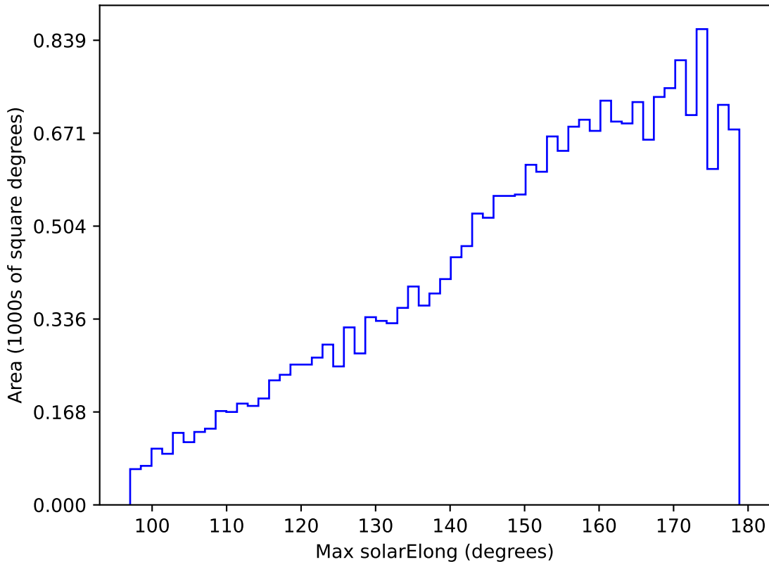
roll_uniform_early_half_mjdp0_v3.4_10yrs All sky u band: Max solarElong
