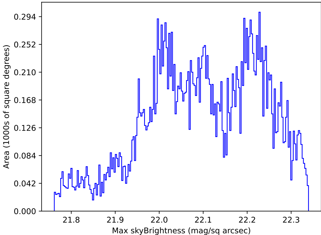
roll_uniform_early_half_mjdp0_v3.4_10yrs Yr 1 g band: Max skyBrightness
