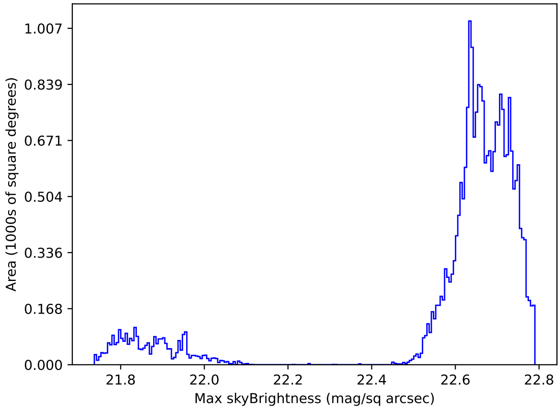
roll_uniform_early_half_mjdp0_v3.4_10yrs Yr 1 all bands: Max skyBrightness
