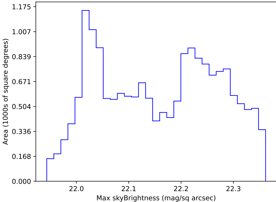
roll_uniform_early_half_mjdp0_v3.4_10yrs WFD g band: Max skyBrightness
