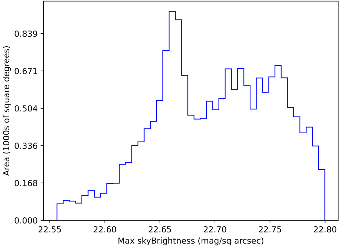
roll_uniform_early_half_mjdp0_v3.4_10yrs WFD all bands: Max skyBrightness
