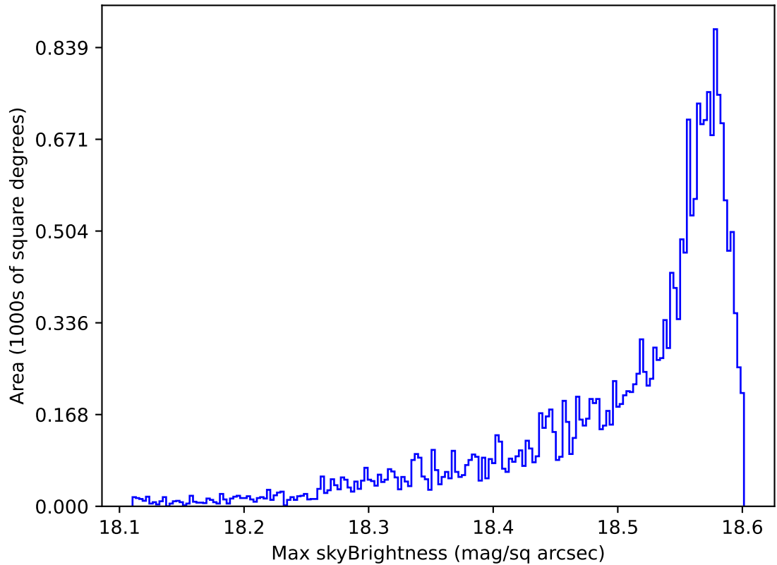
roll_uniform_early_half_mjdp0_v3.4_10yrs All sky y band: Max skyBrightness
