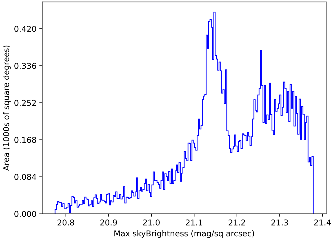
roll_uniform_early_half_mjdp0_v3.4_10yrs All sky r band: Max skyBrightness
