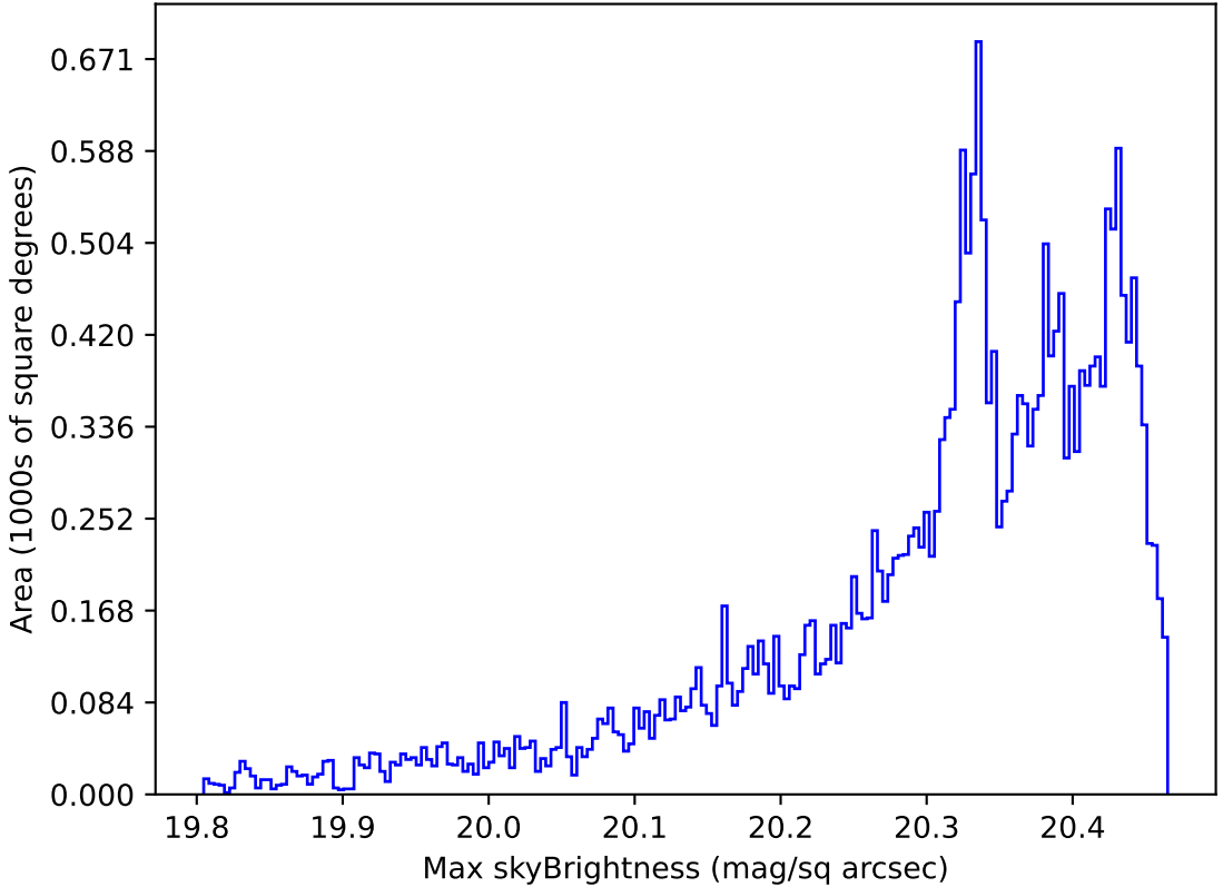
roll_uniform_early_half_mjdp0_v3.4_10yrs All sky i band: Max skyBrightness
