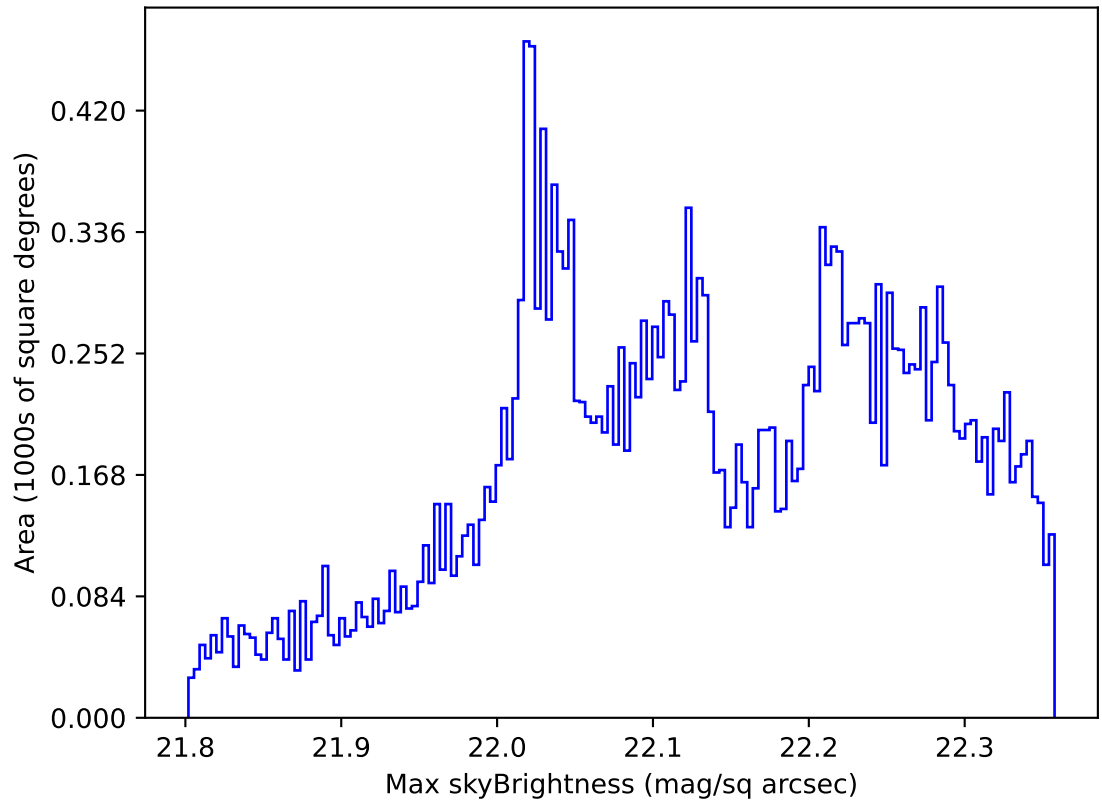
roll_uniform_early_half_mjdp0_v3.4_10yrs All sky g band: Max skyBrightness
