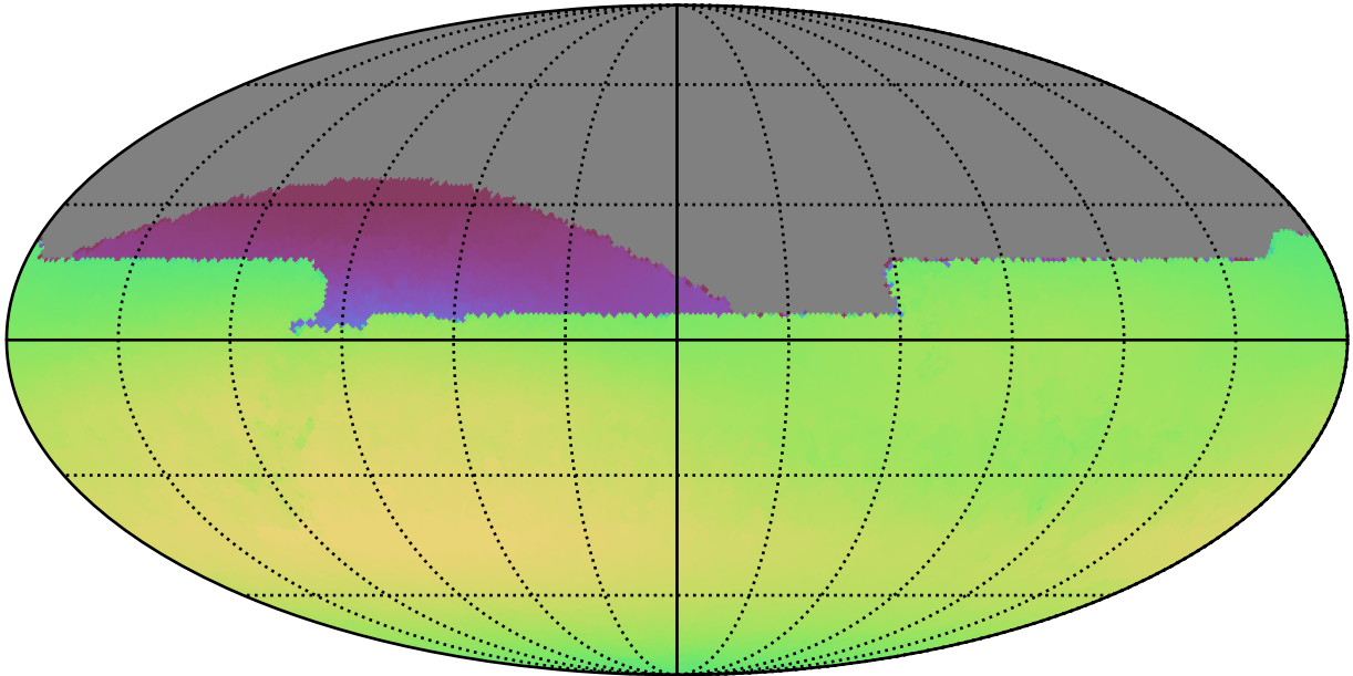
roll_uniform_early_half_mjdp0_v3.4_10yrs All sky all bands: Max skyBrightness
