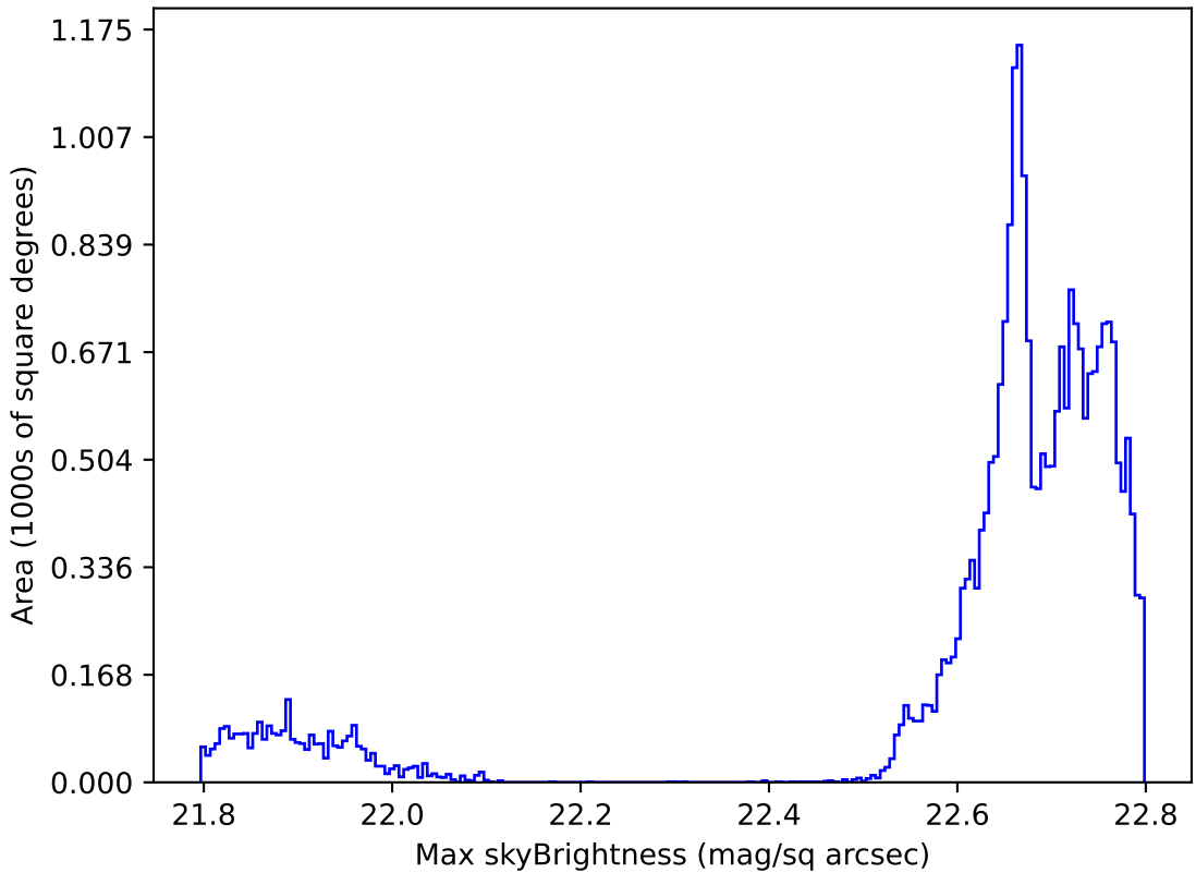
roll_uniform_early_half_mjdp0_v3.4_10yrs All sky all bands: Max skyBrightness
