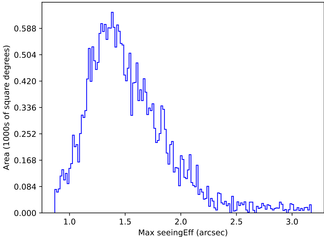
roll_uniform_early_half_mjdp0_v3.4_10yrs Yr 1 z band: Max seeingEff
