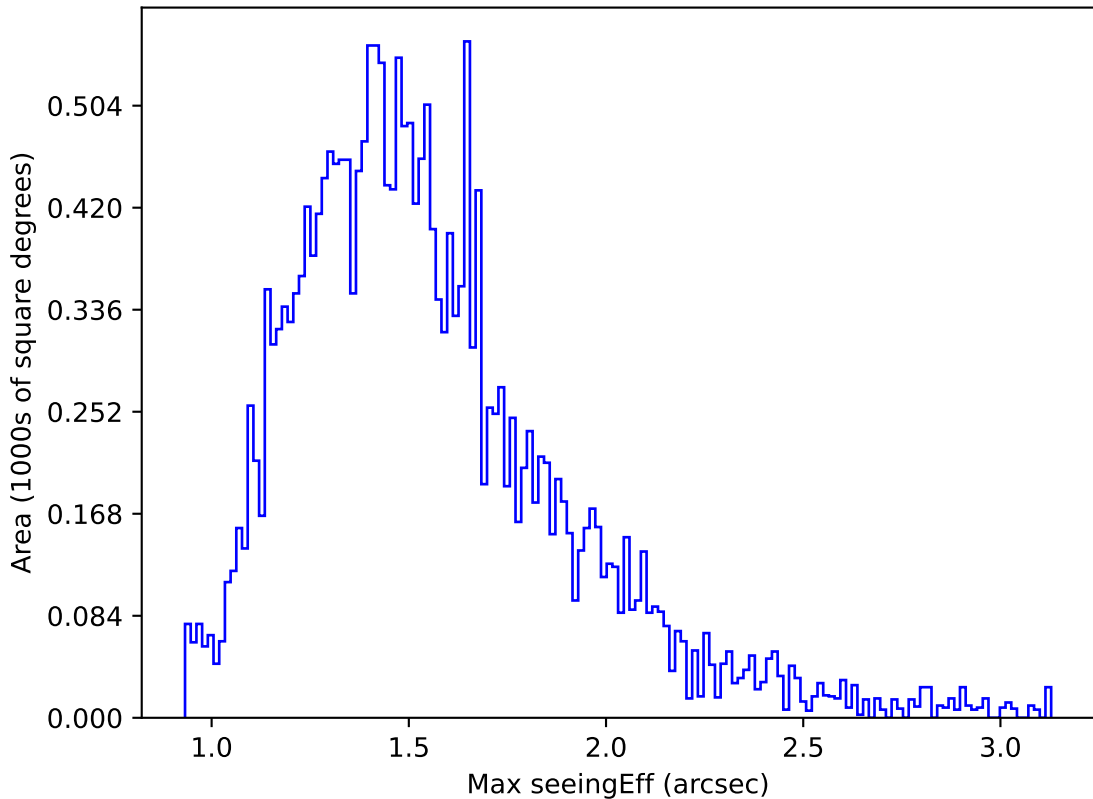
roll_uniform_early_half_mjdp0_v3.4_10yrs Yr 1 u band: Max seeingEff
