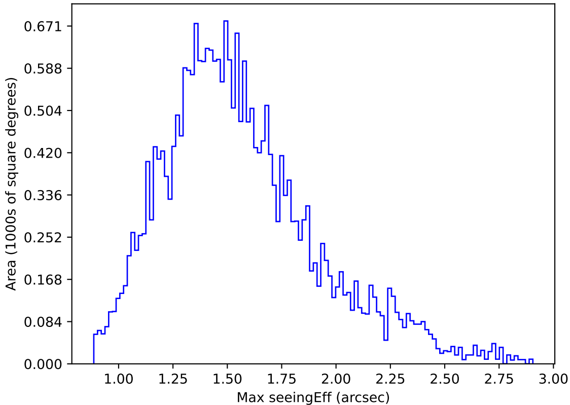
roll_uniform_early_half_mjdp0_v3.4_10yrs Yr 1 r band: Max seeingEff
