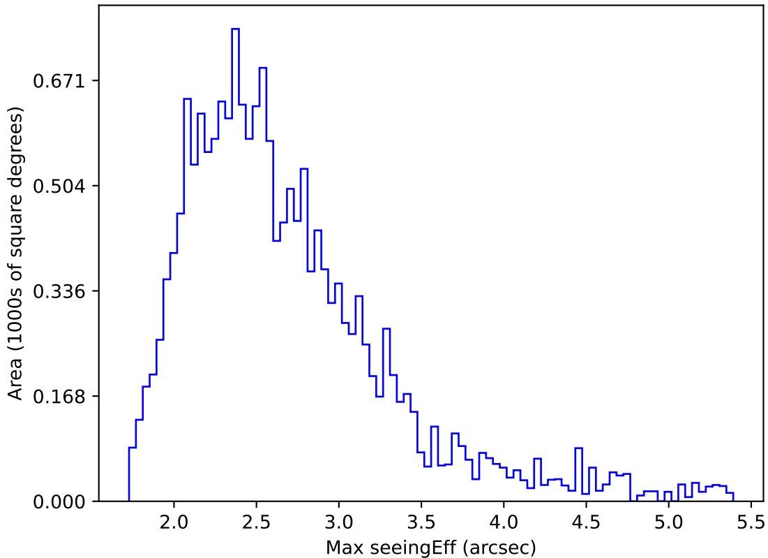
roll_uniform_early_half_mjdp0_v3.4_10yrs WFD i band: Max seeingEff
