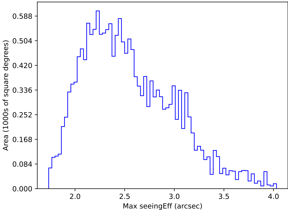
roll_uniform_early_half_mjdp0_v3.4_10yrs WFD g band: Max seeingEff
