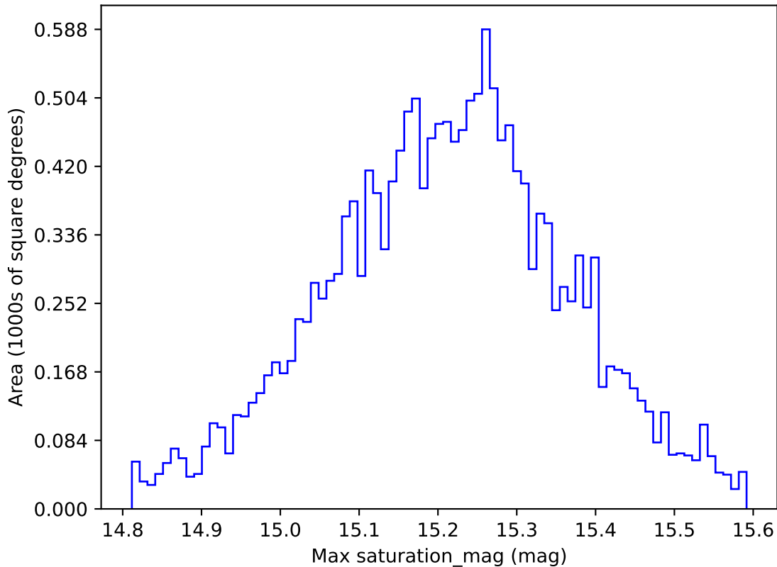
roll_uniform_early_half_mjdp0_v3.4_10yrs WFD z band: Max saturation_mag
