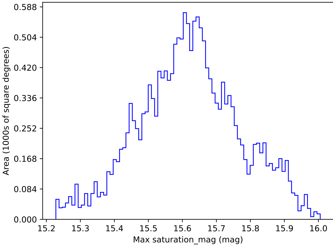
roll_uniform_early_half_mjdp0_v3.4_10yrs WFD i band: Max saturation_mag
