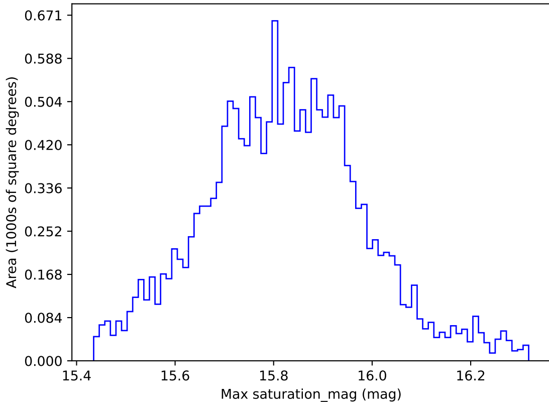
roll_uniform_early_half_mjdp0_v3.4_10yrs WFD all bands: Max saturation_mag
