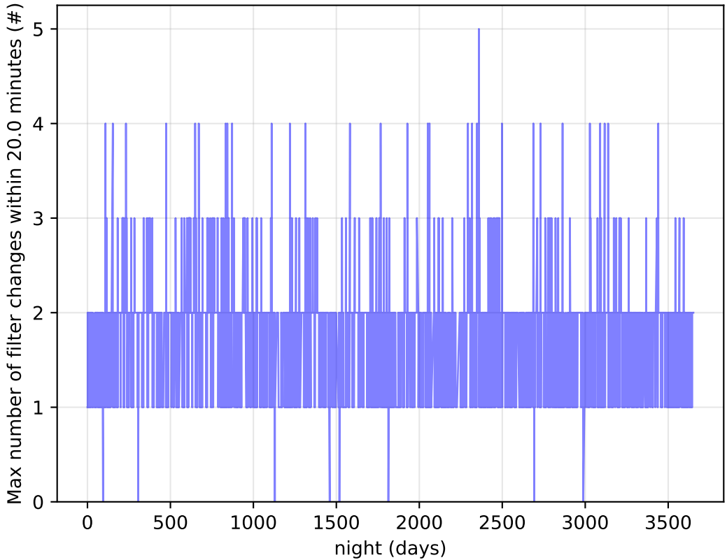
roll_uniform_early_half_mjdp0_v3.4_10yrs Per Night: Max number of filter changes within 20.0 minutes
