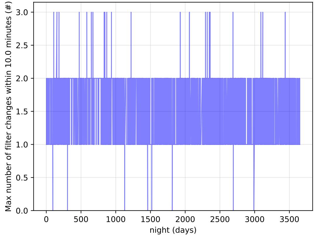
roll_uniform_early_half_mjdp0_v3.4_10yrs Per Night: Max number of filter changes within 10.0 minutes
