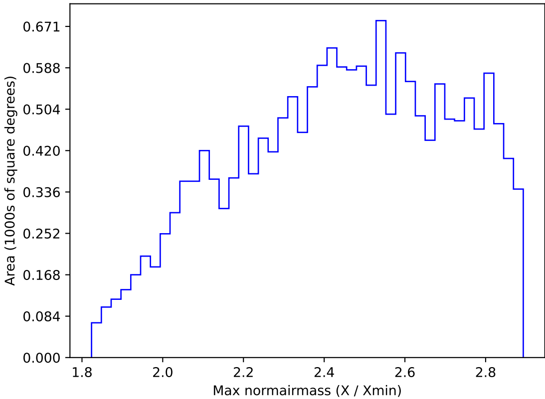
roll_uniform_early_half_mjdp0_v3.4_10yrs WFD all bands: Max normairmass
