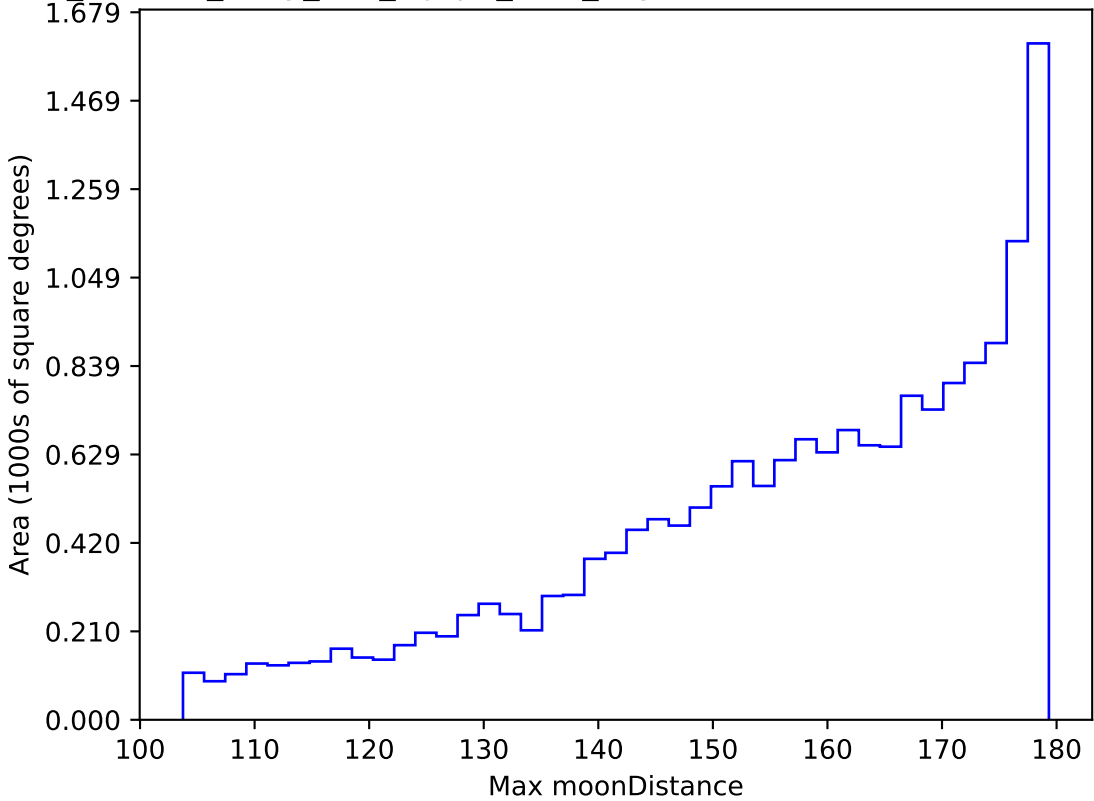
roll_uniform_early_half_mjdp0_v3.4_10yrs WFD r band: Max moonDistance
