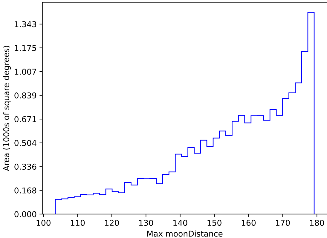
roll_uniform_early_half_mjdp0_v3.4_10yrs WFD i band: Max moonDistance
