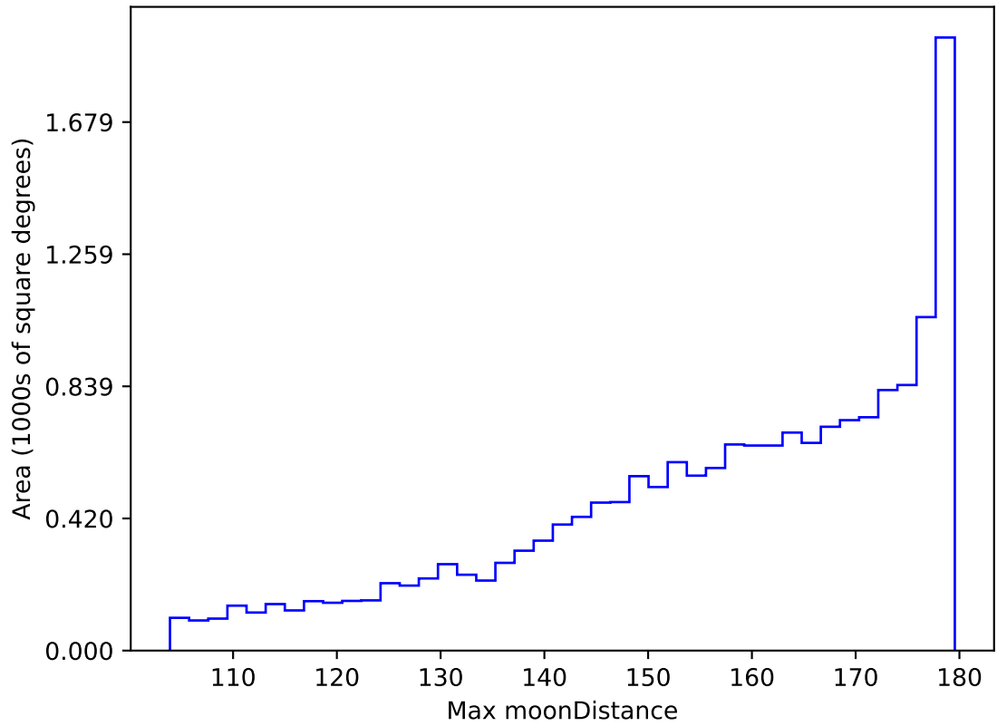
roll_uniform_early_half_mjdp0_v3.4_10yrs WFD all bands: Max moonDistance
