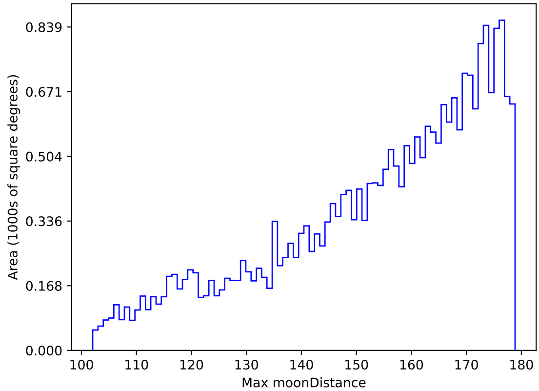
roll_uniform_early_half_mjdp0_v3.4_10yrs All sky z band: Max moonDistance
