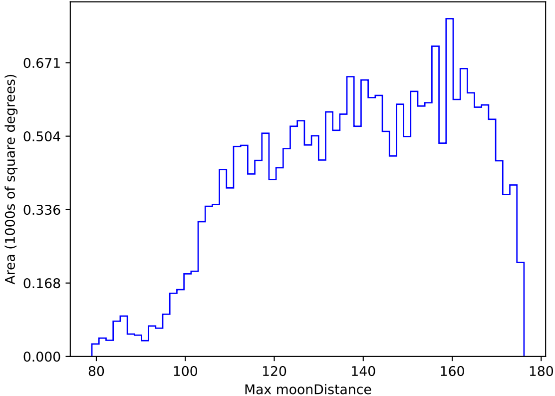
roll_uniform_early_half_mjdp0_v3.4_10yrs All sky y band: Max moonDistance
