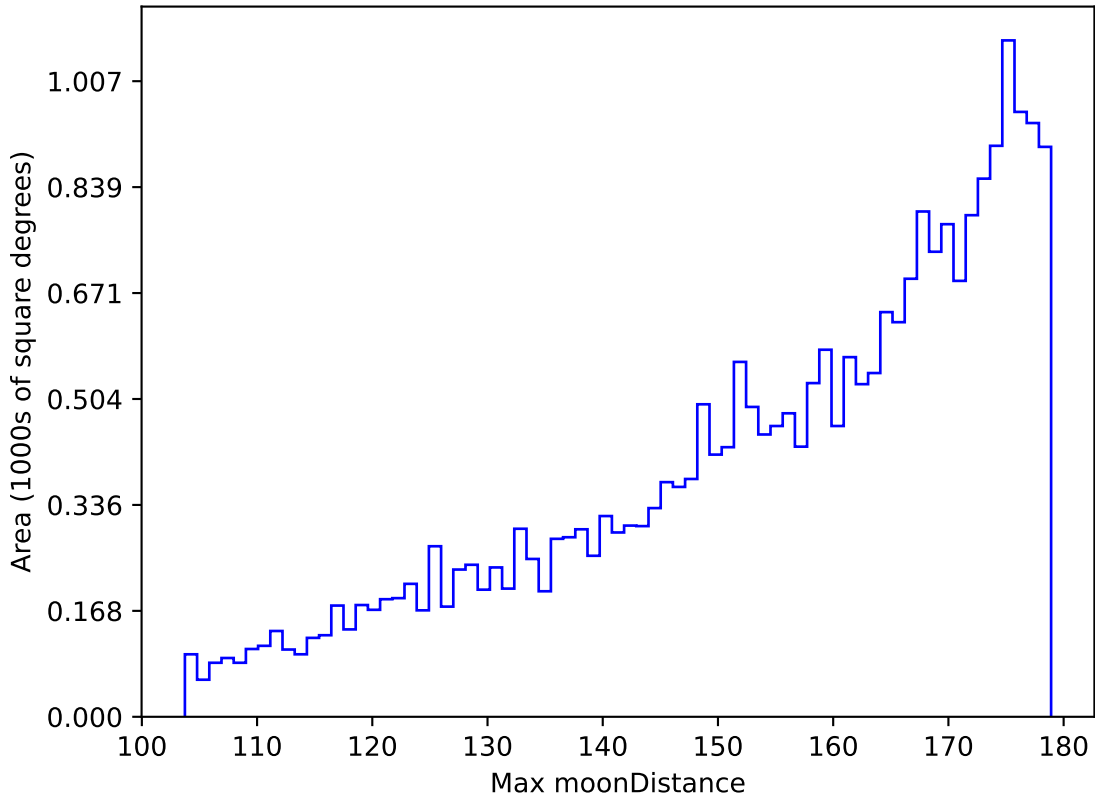
roll_uniform_early_half_mjdp0_v3.4_10yrs All sky g band: Max moonDistance
