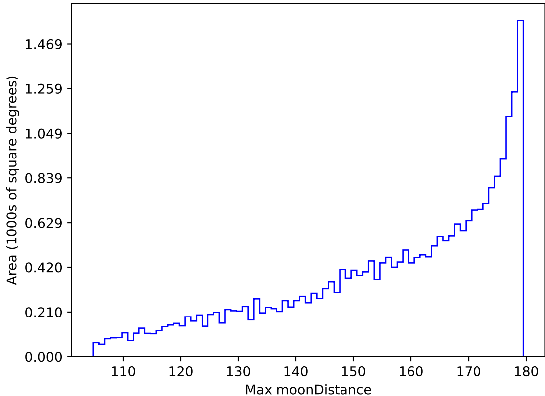
roll_uniform_early_half_mjdp0_v3.4_10yrs All sky all bands: Max moonDistance
