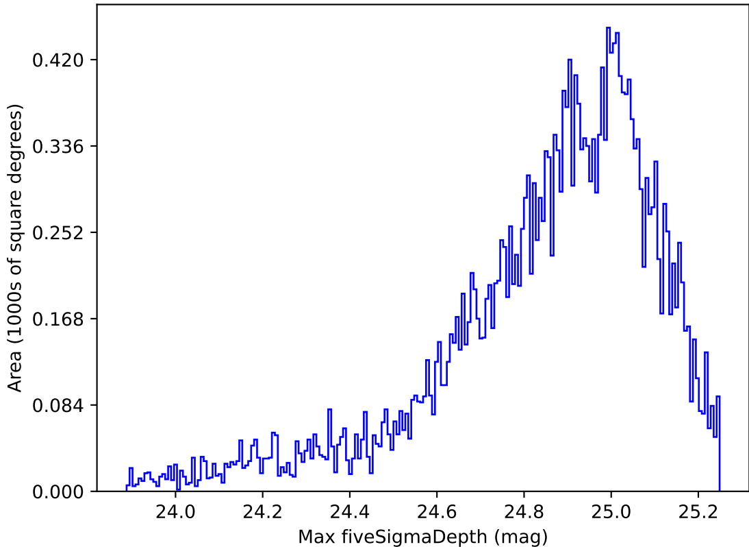
roll_uniform_early_half_mjdp0_v3.4_10yrs Yr 1 all bands: Max fiveSigmaDepth
