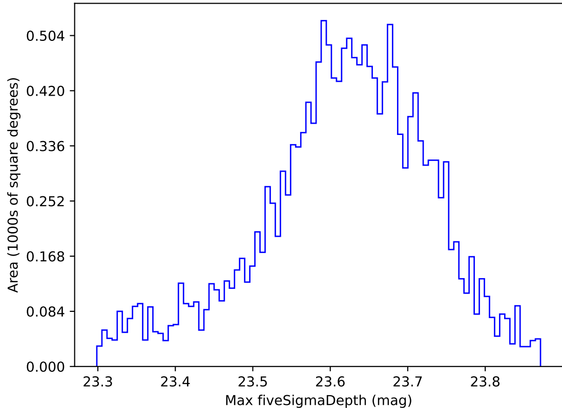
roll_uniform_early_half_mjdp0_v3.4_10yrs WFD z band: Max fiveSigmaDepth
