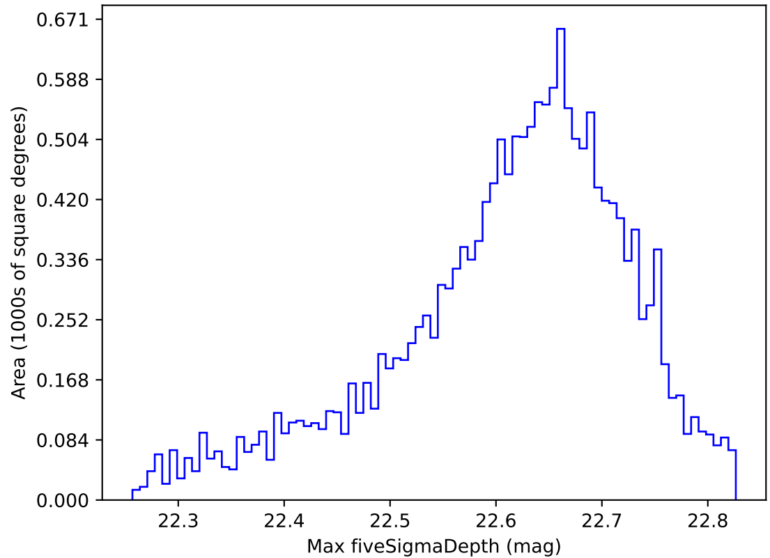
roll_uniform_early_half_mjdp0_v3.4_10yrs WFD y band: Max fiveSigmaDepth
