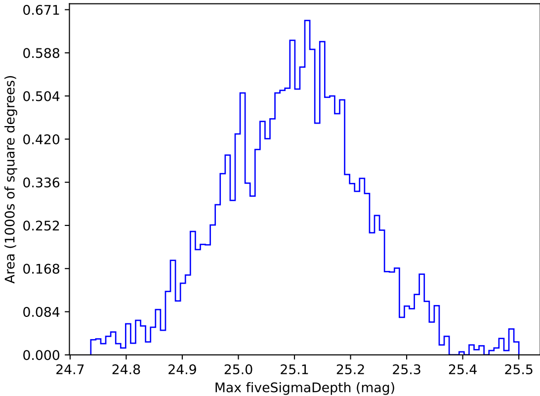
roll_uniform_early_half_mjdp0_v3.4_10yrs WFD g band: Max fiveSigmaDepth
