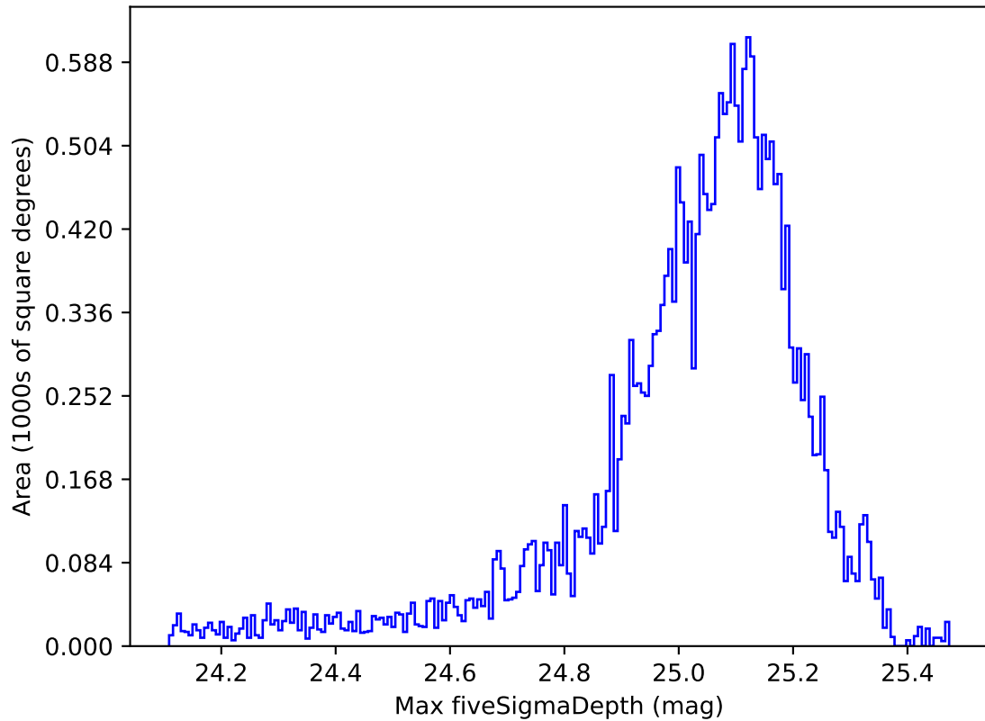
roll_uniform_early_half_mjdp0_v3.4_10yrs All sky all bands: Max fiveSigmaDepth
