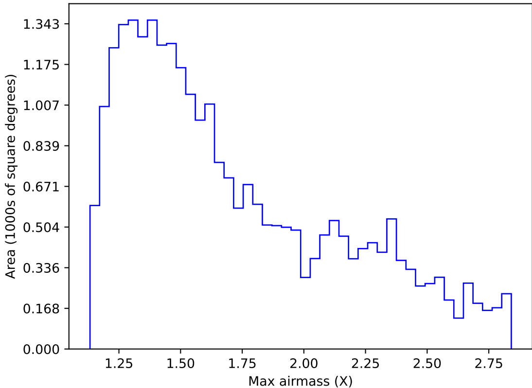
roll_uniform_early_half_mjdp0_v3.4_10yrs Yr 1 i band: Max airmass
