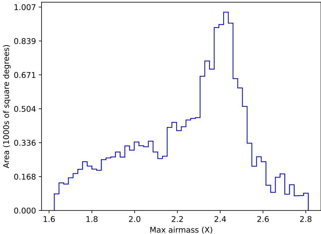
roll_uniform_early_half_mjdp0_v3.4_10yrs WFD r band: Max airmass
